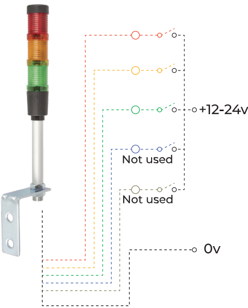
Wiring Diagram 2 (BR100)
